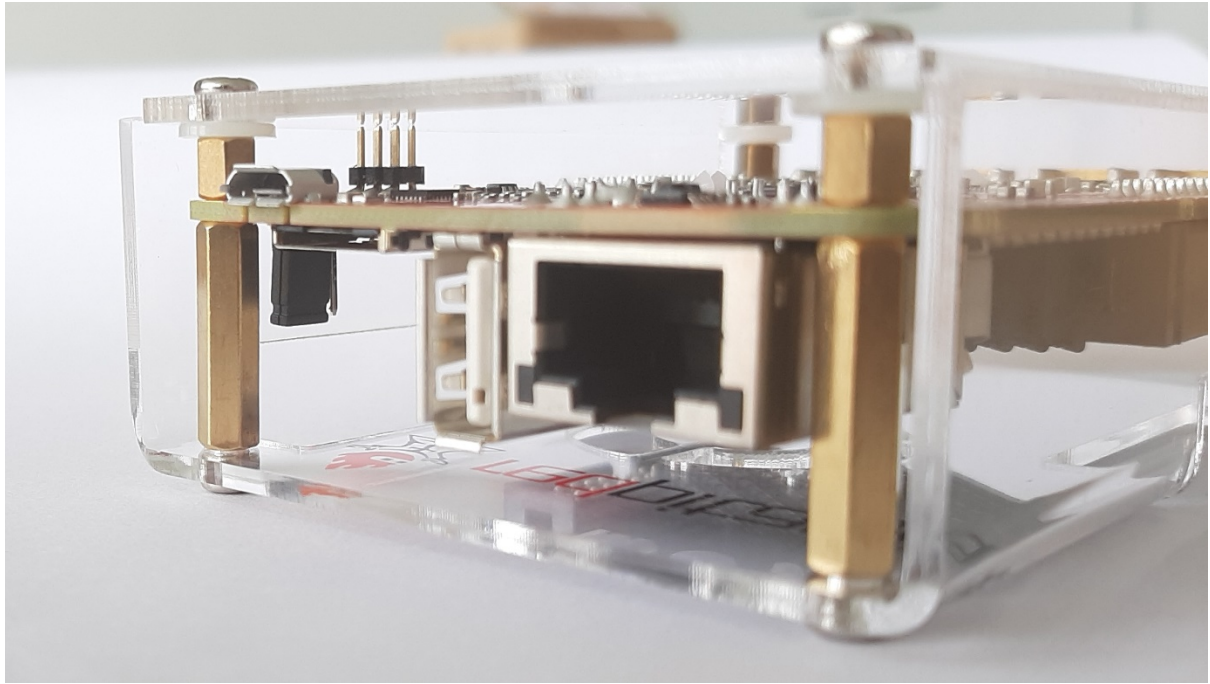
Red Pitaya showing use of white plastic washers for 6-pin connector CN11 clearance
