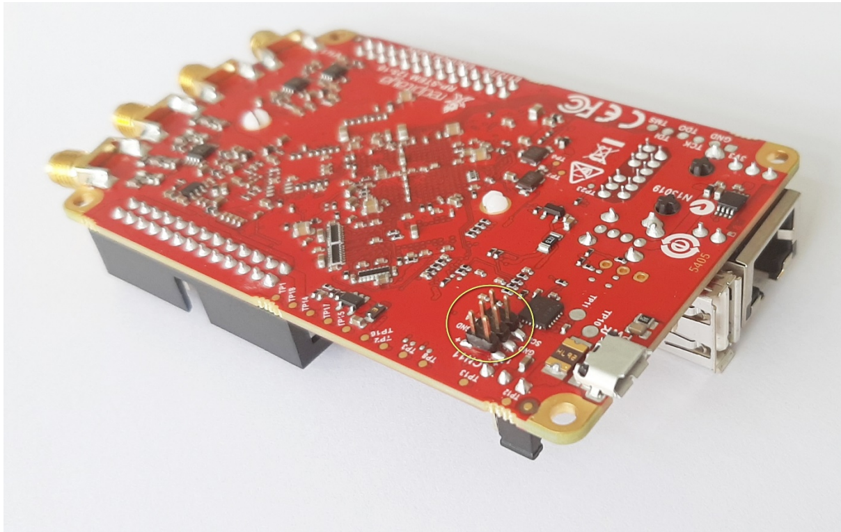
Red Pitaya bottom pcb showing the 6-pin connector CN11
